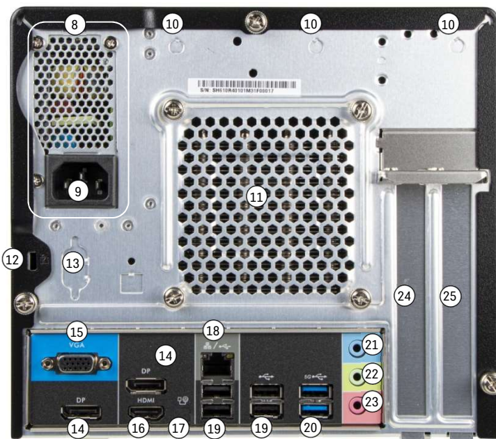
Back panel
